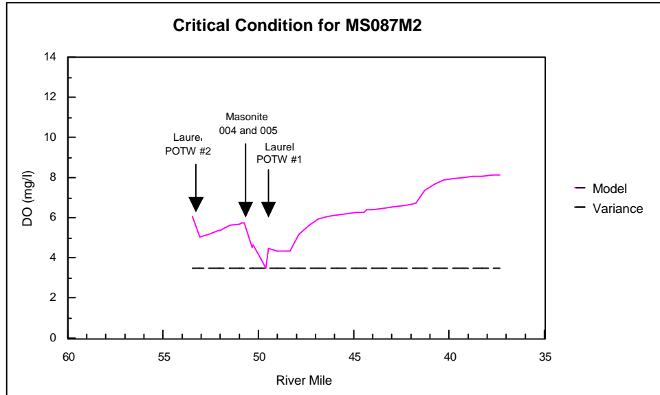
Figure 3. Model results for the critical condition in Segment MS087M2
