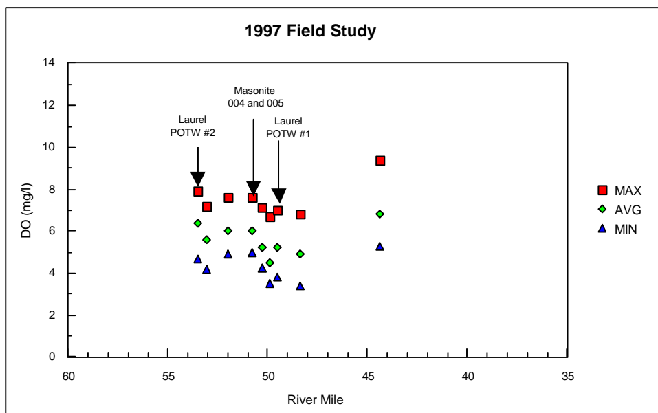
Figure 2. 1997 Field Study: Daily Maximum, Average, and Minimum Measured DOs
