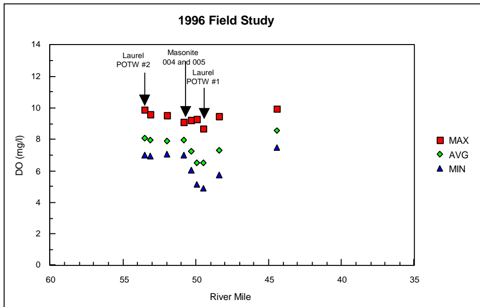
Figure 1. 1996 Field Study: Daily Maximum, Average, and Minimum Measured Dos
